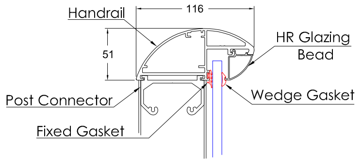
DETAILED VIEW : HANDRAIL
